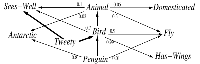
Figure 1: A graphical representation of a knowledge base
