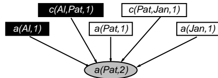
Fig. 3. Simple query for the AIDS knowledge base
